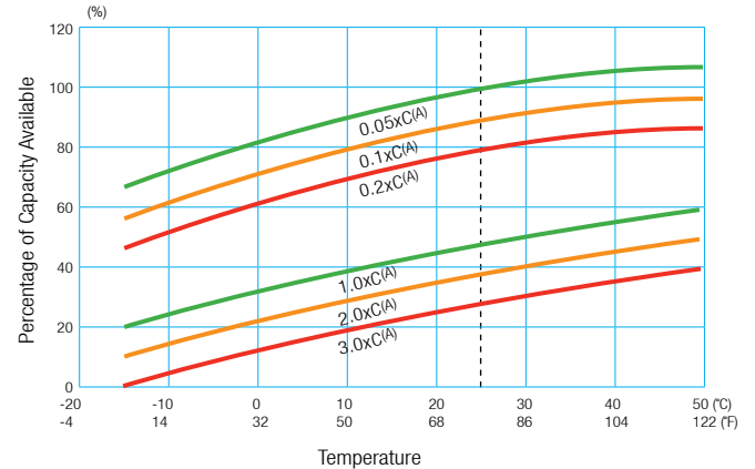
Temperature Effects in Relation to Battery Capacity
